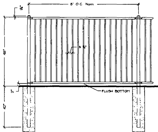
ORNAMENTAL FENCE DETAIL NOT TO SCALE
