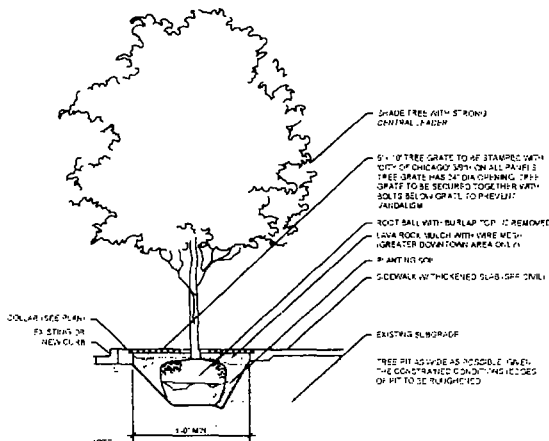
3 SHADE TREE IN GRATE SECTION NOT TO SCALE
