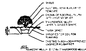
4 SHRUB PLANTING SECTION NOT TO SCALE
