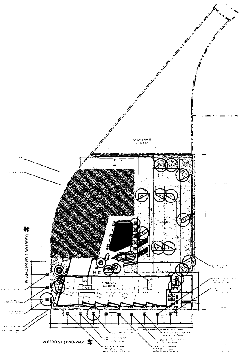
1 OVERALL SITE PLAN 1" = 20'-0"
