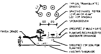
5 PERENNIAL PLANTING SECTION NOT TO SCALE
