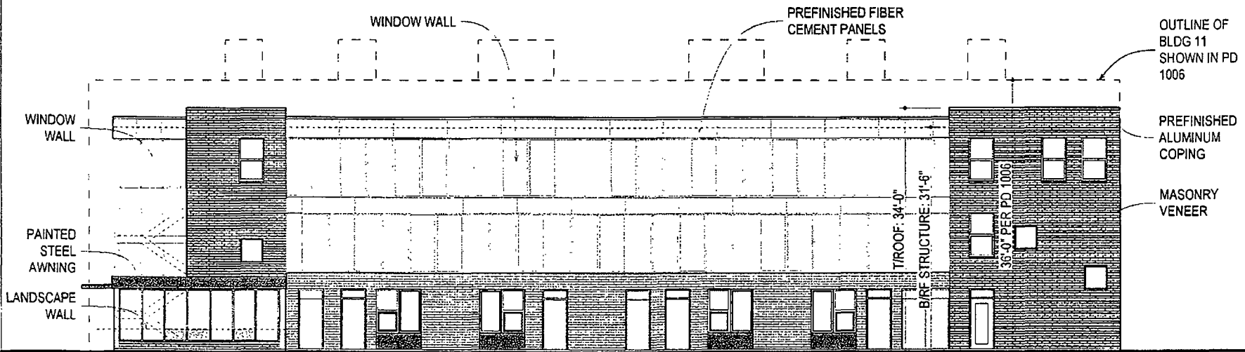
1 SOUTH ELEVATION SCALE 3/32" = 1'-0"
