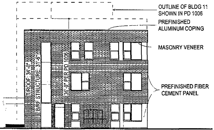
2 EAST ELEVATION SCALE: 3/32" = 1'-0" 0 8' 16' 24'
