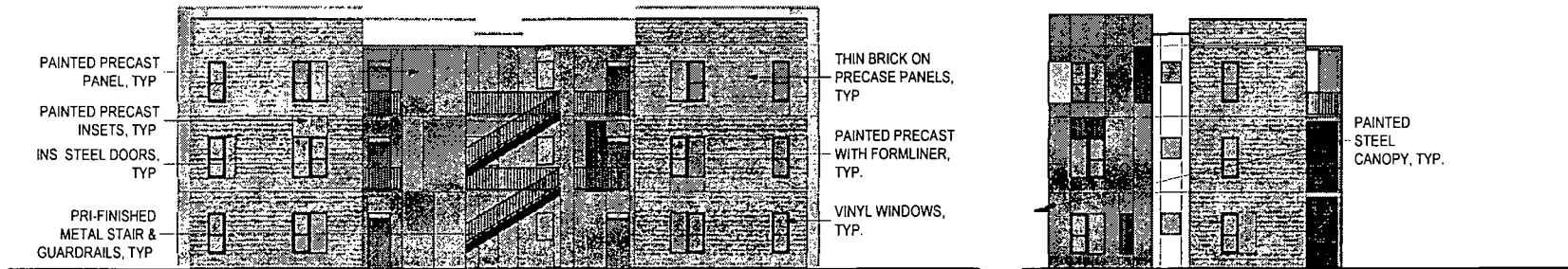
1 EXTERIOR ELEVATION: Building 16 Rear SCALE 1/16" = 1'-0"
