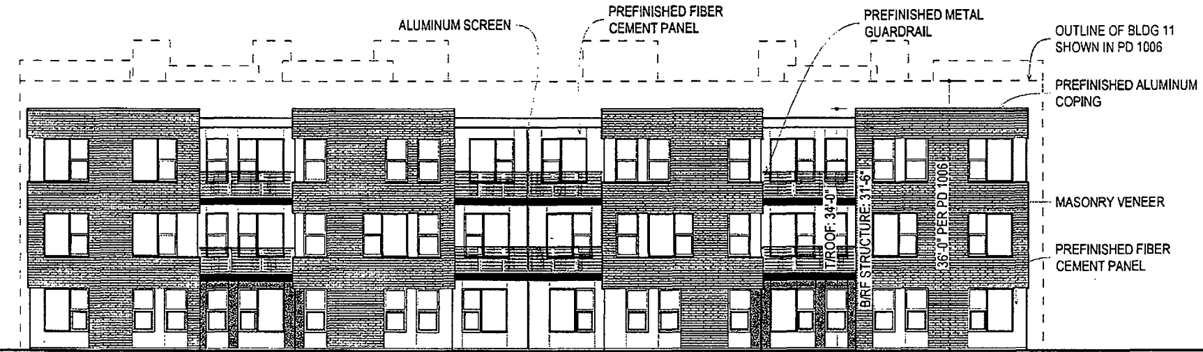
1 NORTH ELEVATION SCALE: 3/32" = 1'-0"
