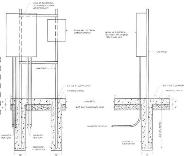
LIGHTING CONTROLLER MOUNTING-FRONT VIEW
