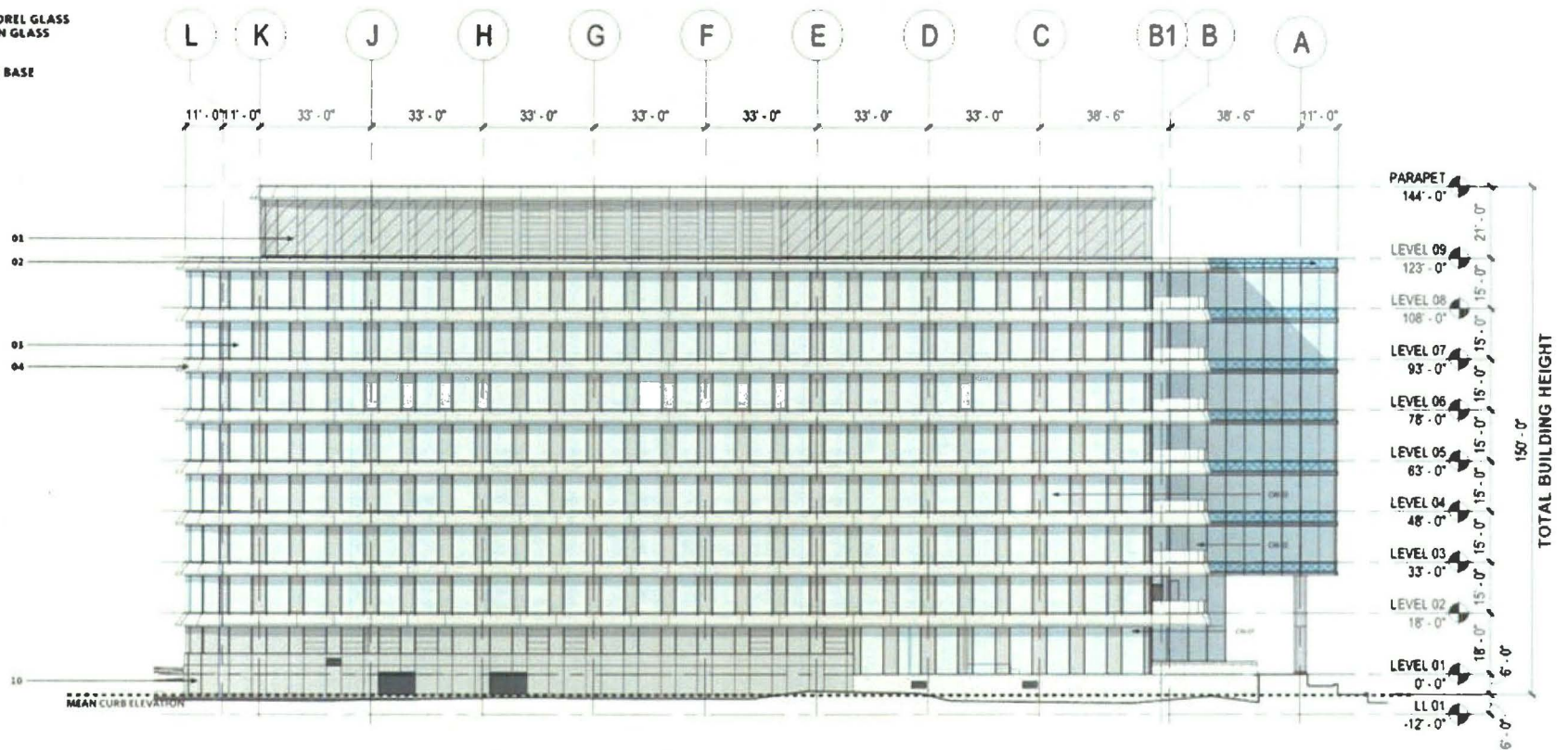
01 ELEVATION SOUTH
