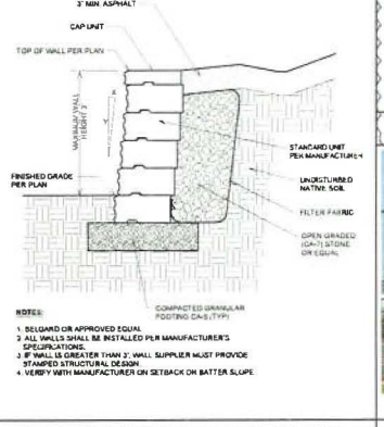
TYPICAL SEGMENTED BLOCK WALL SECTION
