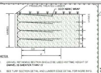
GRAVEL RETAINING SECTION
