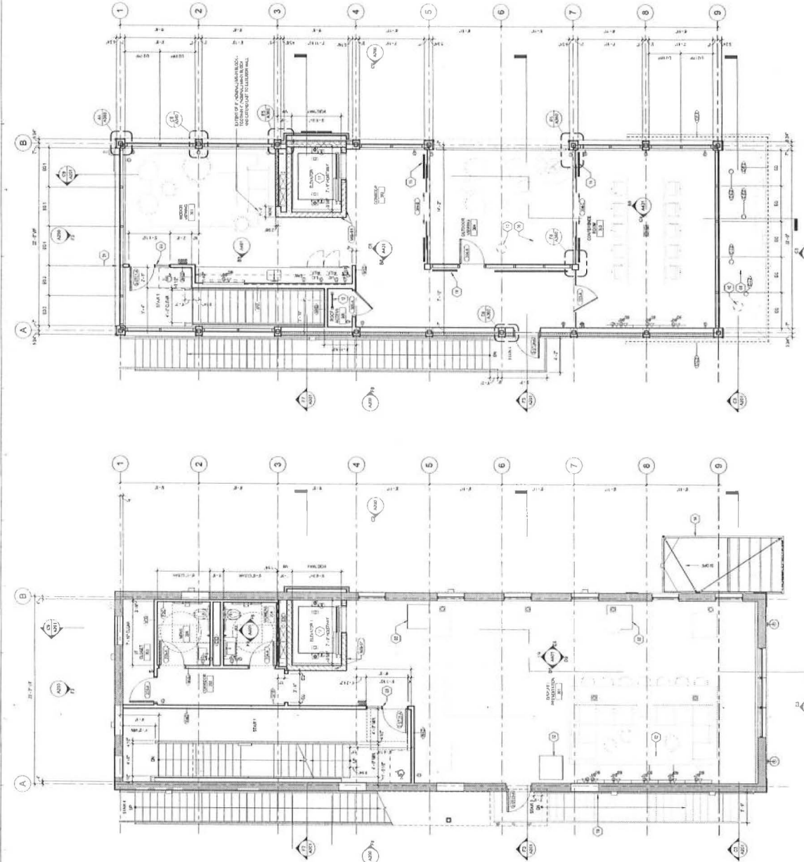
F5 FLOOR PLAN - LEVEL 3
