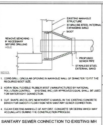
SANITARY SEWER CONNECTION TO EXISTING MH
