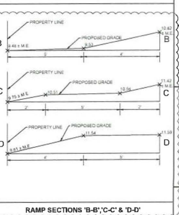
RAMP SECTIONS 'B-B', 'C-C' & 'D-D'
