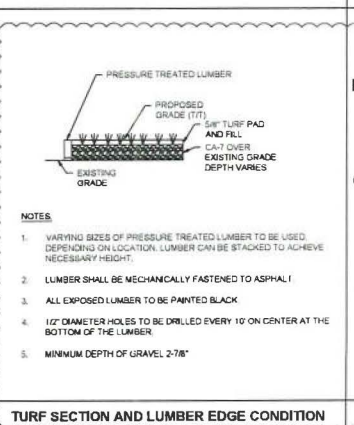
TURF SECTION AND LUMBER EDGE CONDITION
