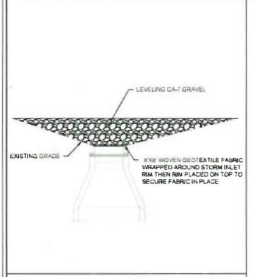
INLET PROTECTION AND LEVELING
