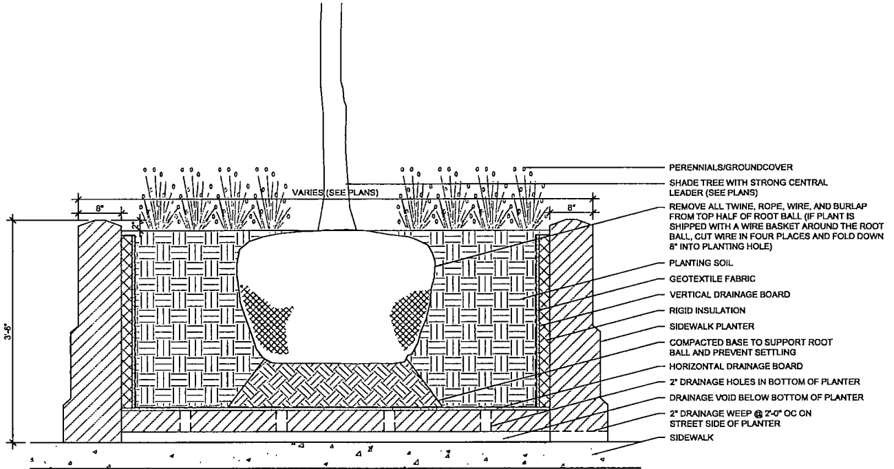
1 SIDEWALK PLANTER W/TREE SECTION 1/2" = 1'-0"
