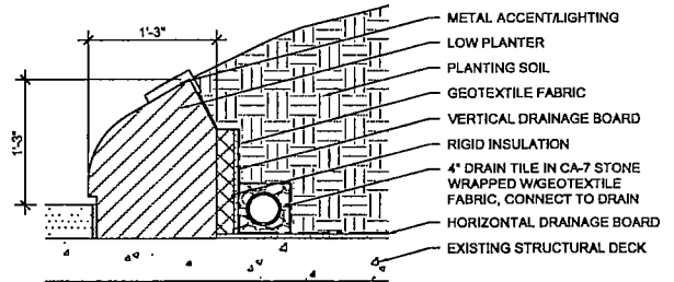
3 LOW PLANTER SECTION 1/2" = 1'-0"
