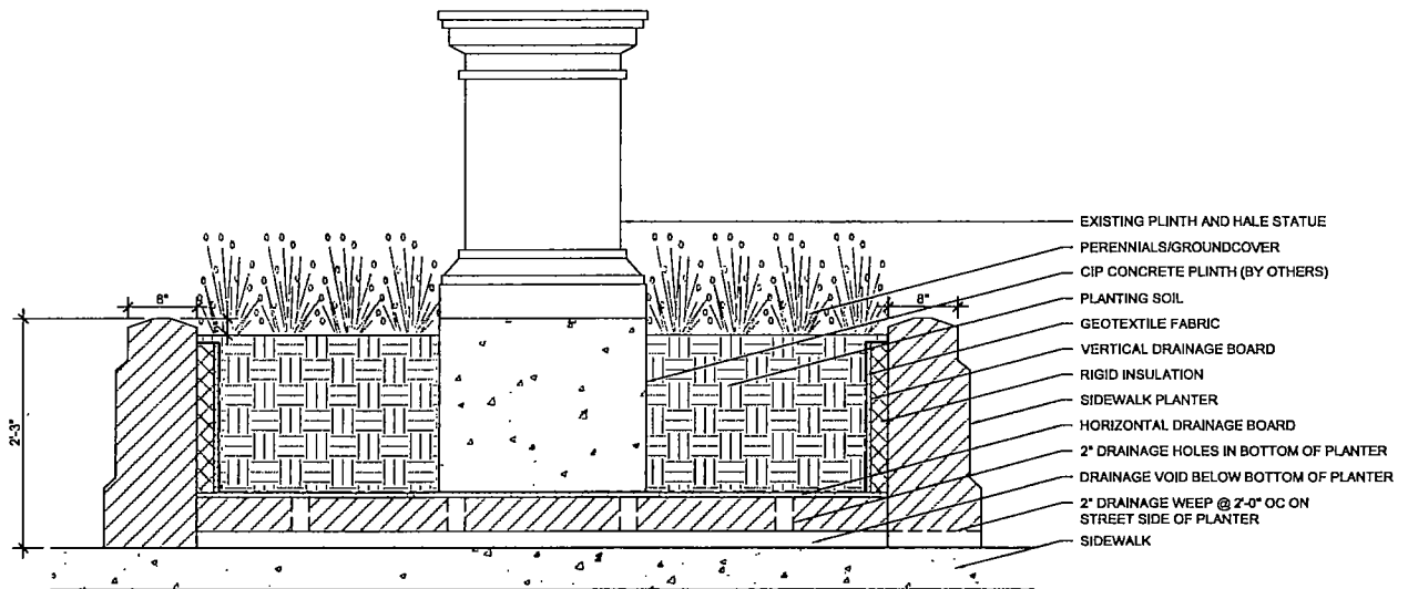
2 SIDEWALK PLANTER W/STATUE SECTION 1/2" = 1'-0"
