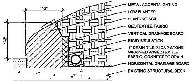
2 LOW PLANTER SECTION 1/2" = 1'-0"
