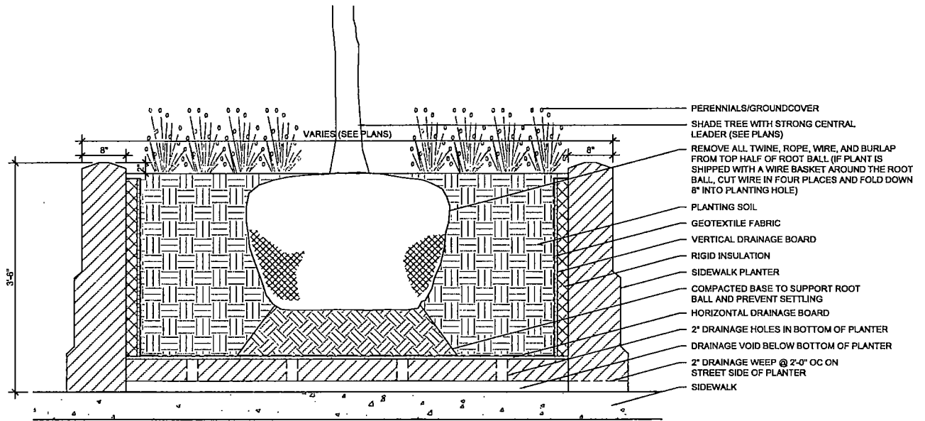
1 SIDEWALK PLANTER W/TREE SECTION 1/2" = 1'-0"
