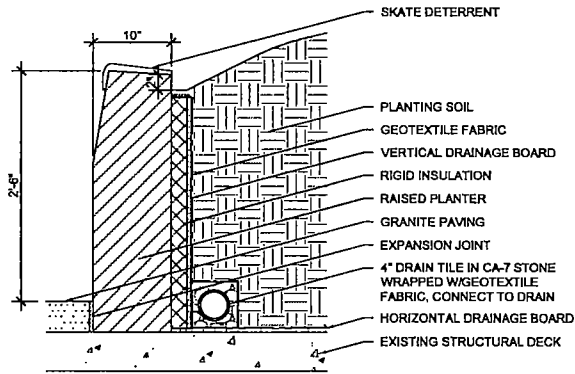
1 RAISED PLANTER SECTION 1/2" = 1'-0"
