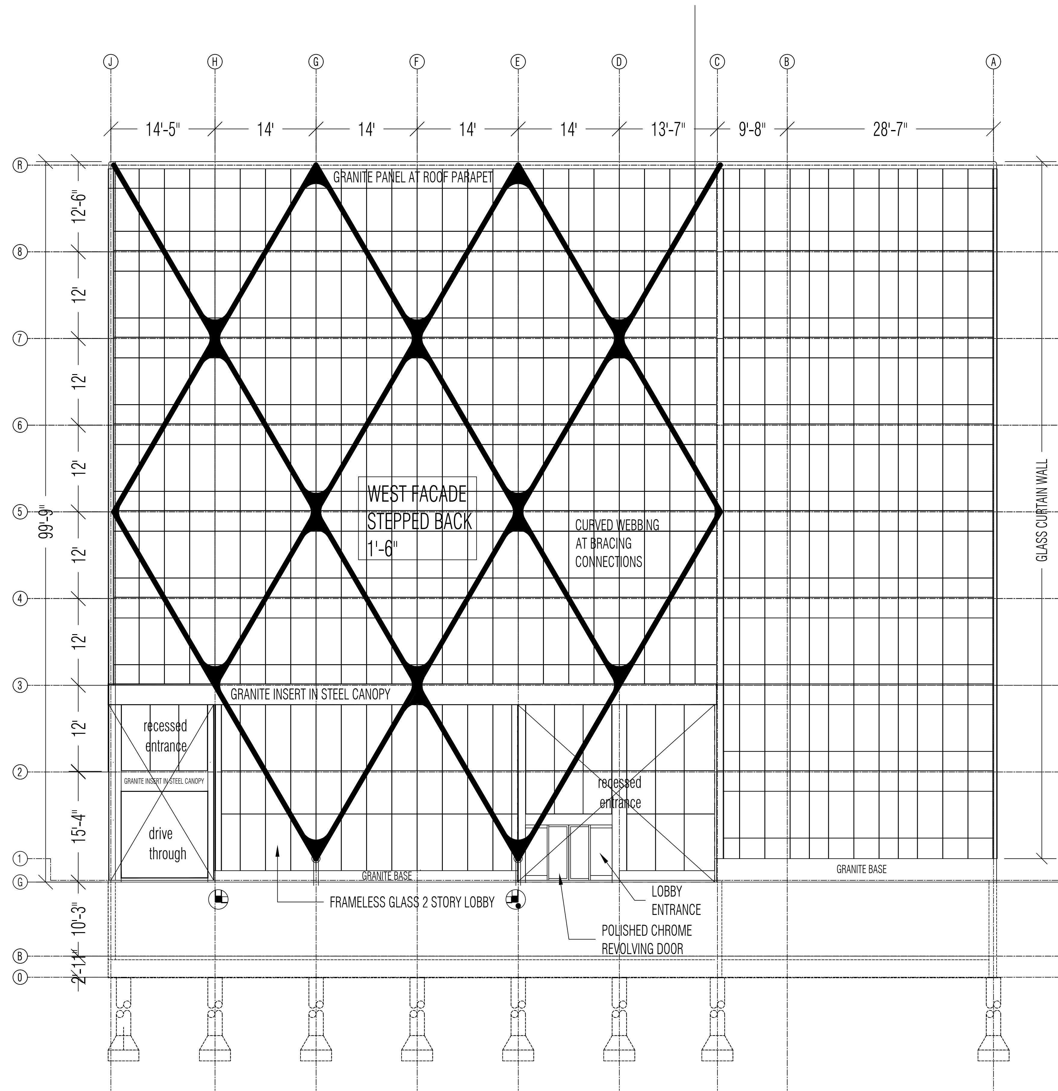
1 SOUTH ELEVATION Scale: 1/8" = 1'-0" 10 0 4 8 20
