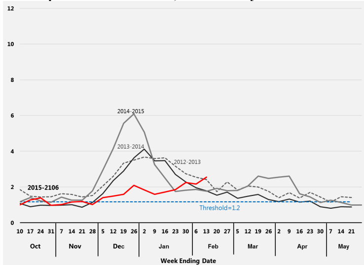
Figure 4. Percent of medically attended outpatient visits attributed to influenza-like illness as reported by ILINet facilities, Chicago, by week, for the current season (2015-2016)
